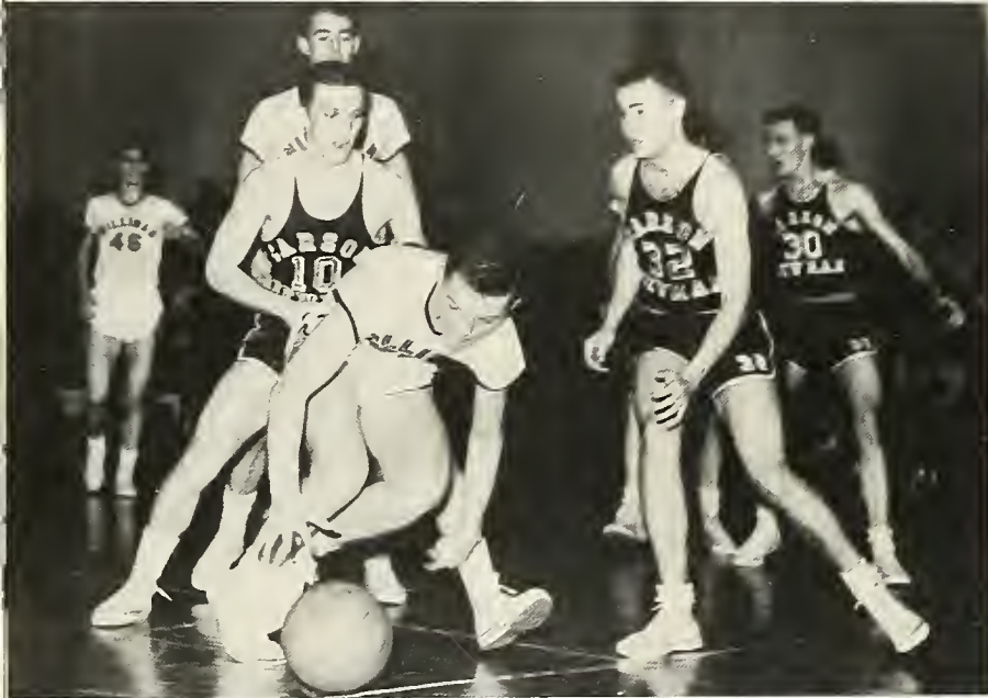
Harris scores.
